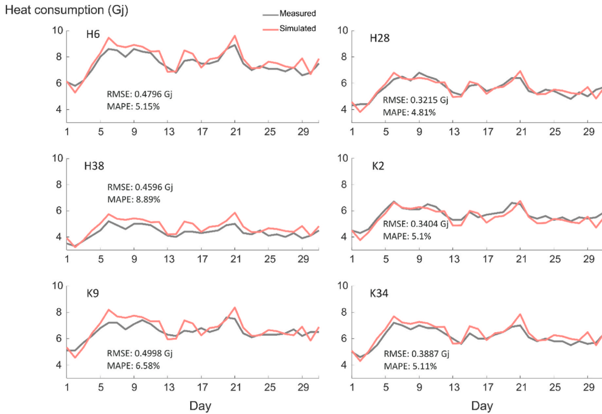
Fig. 6. Model validation results for six substations, conducted in January 2022.
