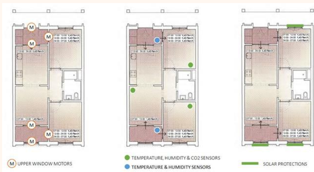
Figure 5. Placement of window motors, sensors and solar protections in an apartment.
