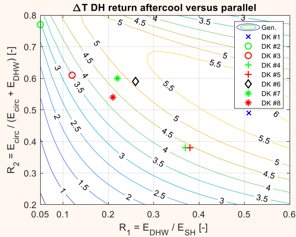
Figure 11. Calculated yearly building level district heating return temperature reduction potential.
