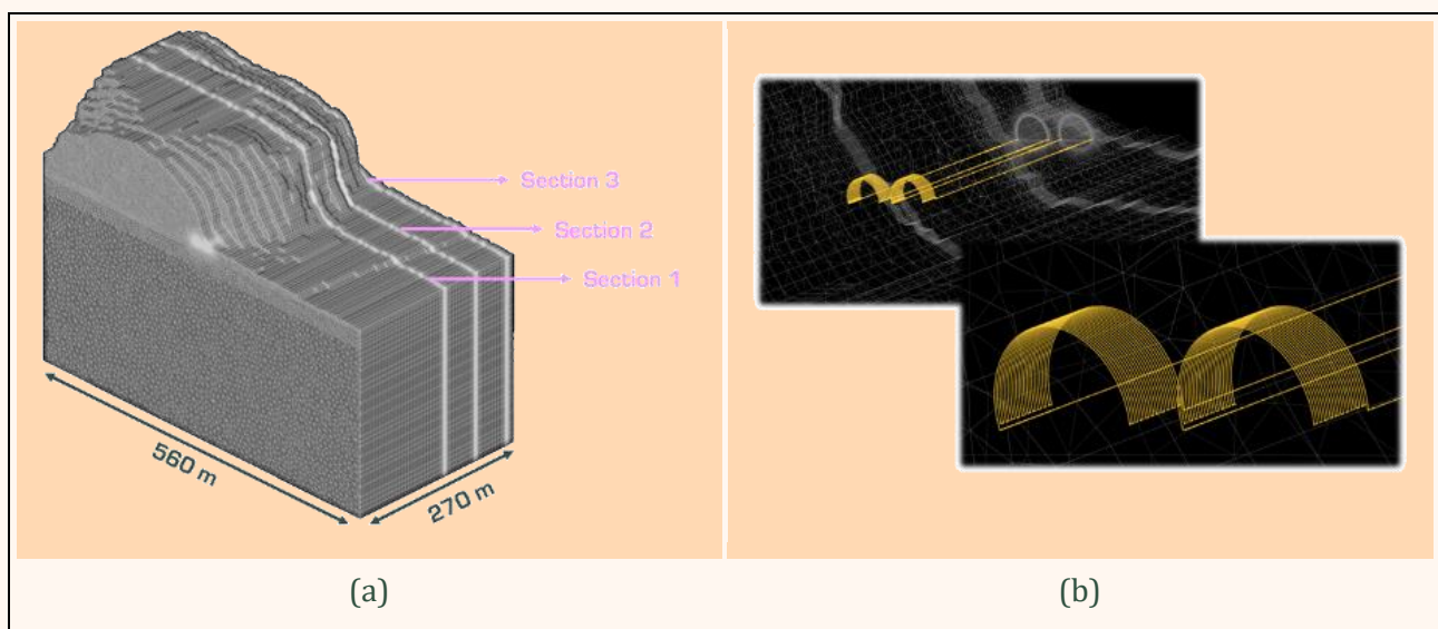
Figure 40. Illustration of (a) the numerical model and (b) close-up view of the heat exchanger system configuration in Section 2 located at an average distance of 65 m from the tunnel mouth.
