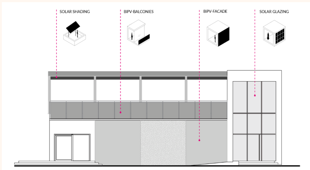
Figure 6. Photovoltaic integration forms identified on the envelope of the Demo Project Trento, South facade. Original graphics by Guido Callegari, Politecnico di Torino.
