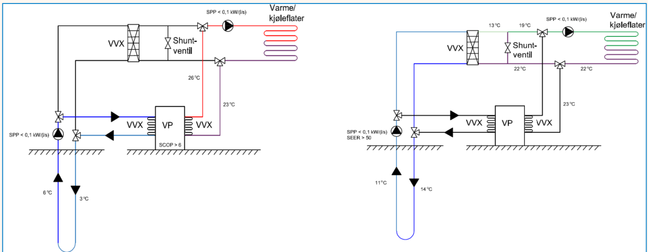
Figure 19. Schematic of the LowEx system, in winter operation (left) and summer operation (right). Source: Tor Helge Dokka, Skanska Norway.
