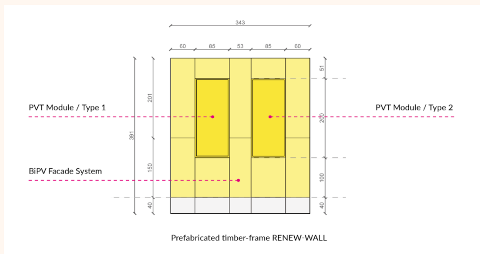
Figure 7. Demo Project Trento, South facade: PVT modules installed in the BIPV facade. Original graphics by Guido Callegari, Politecnico di Torino.
