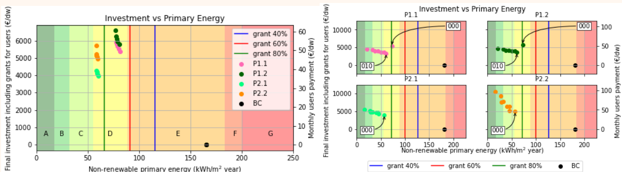
Figure 21. Investment per dwelling vs. non-renewable primary energy use in different renovation scenarios.
