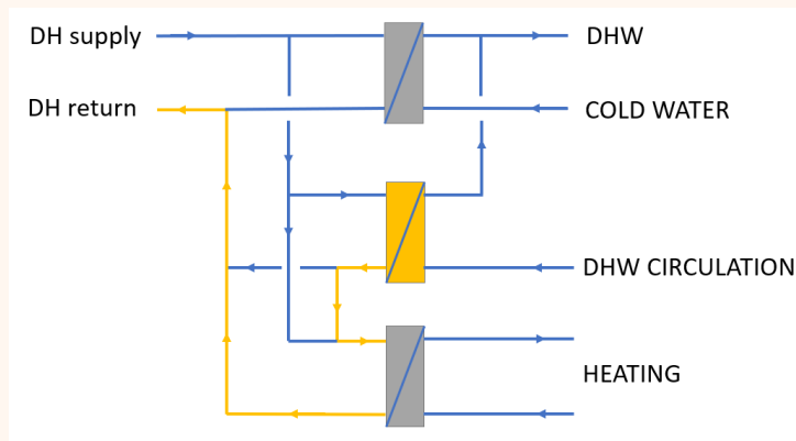
Figure 10. Operating diagram of the aftercooling system
